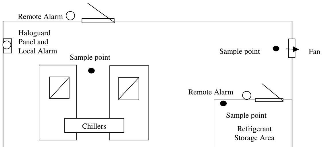
Fig. 1-Typical Area Monitoring Installation
